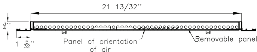
SECTION C-C
